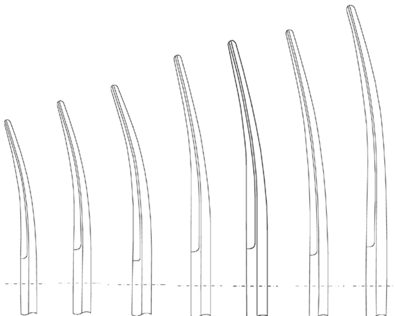
122-101 122-103 122-105 122-107 122-109 122-113 122-115 115mm 130mm 145mm 155mm 165mm 185mm 200mm 4 1/2" 5 1/8" 5 3/4" 6" 6 1/2" 7 1/4" 8" gebogen, curved, curvas, courbes
